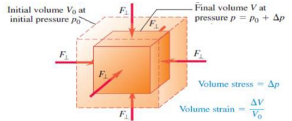
Figure 3.3: A block undergoing volume strain by the applied volume stress
