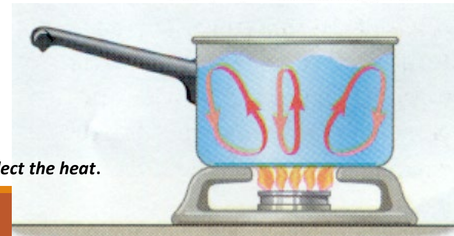
Fig 1 Convection currents
